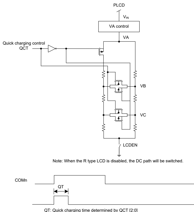
R Type Bias Configuration – 1/3 Bias
