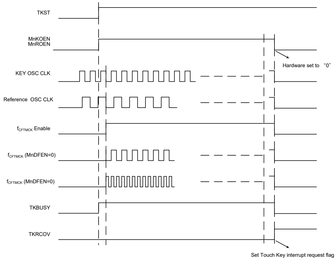
Touch Key Manual Scan Mode Timing Diagram
