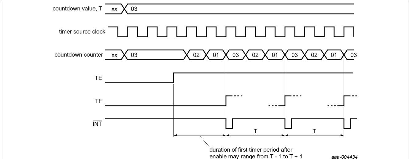
Figure 17. General countdown timer behavior
