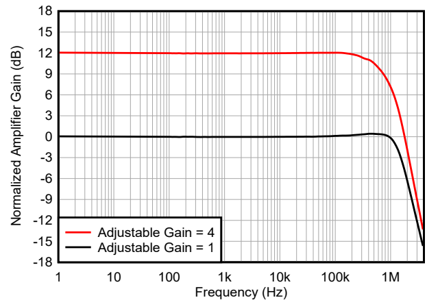
Figure 5-10. Current Sense Amplifier Gain vs Frequency
