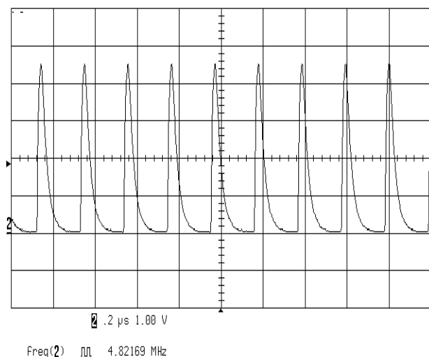
FIGURE 16. SYNC WAVEFORM
