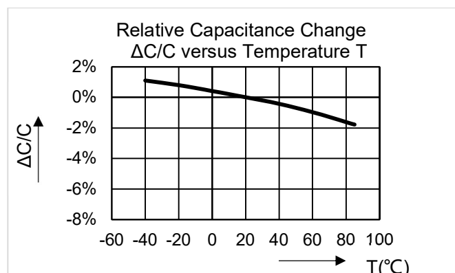
Figure 8: Temperature dependence of capacitance
