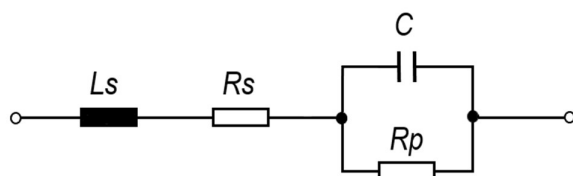
Figure 7: Equivalent circuit diagram
