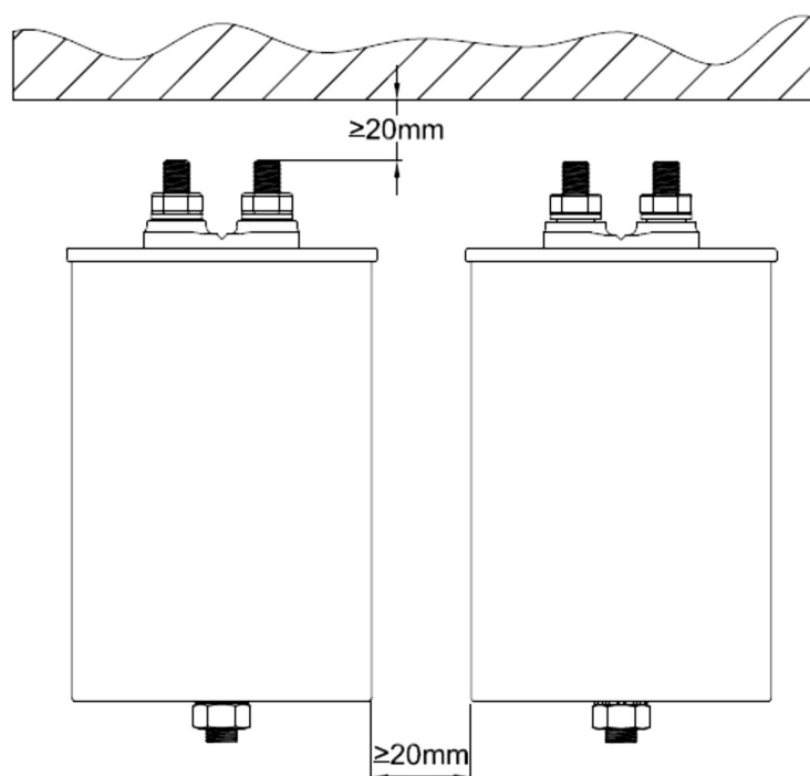
Figure 5: Installation space requirements
