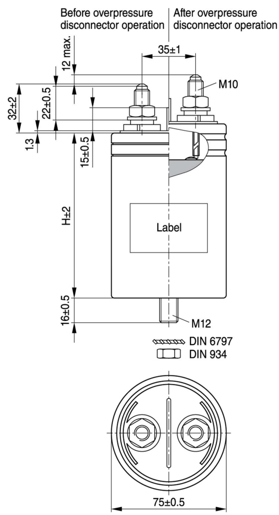
Figure 3: Series B32362 (D = 75 mm)
