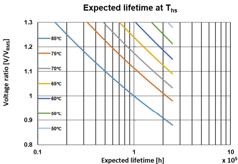
Figure 14: Expected lifetime in hours at different hotspot temperatures ( T_{hs} ) and voltages V_{RMS} .
