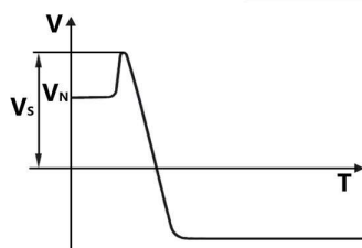
Figure 10: Non-recurrent surge voltage V_s
