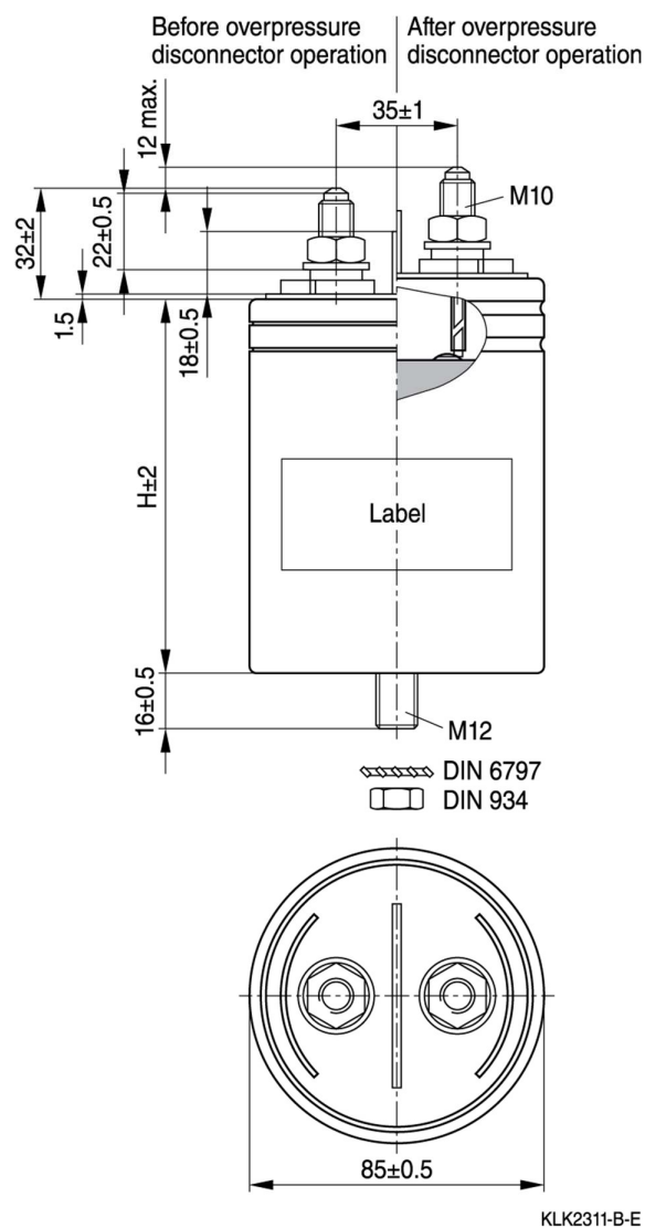
Figure 4: Series B32362 (D = 85 mm)
