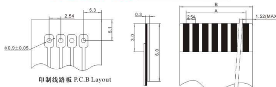
孔座 HOUSING (543)
