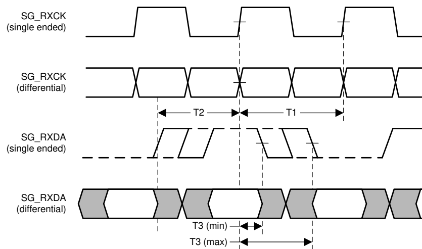
Figure 6-4. SGMII Timing
