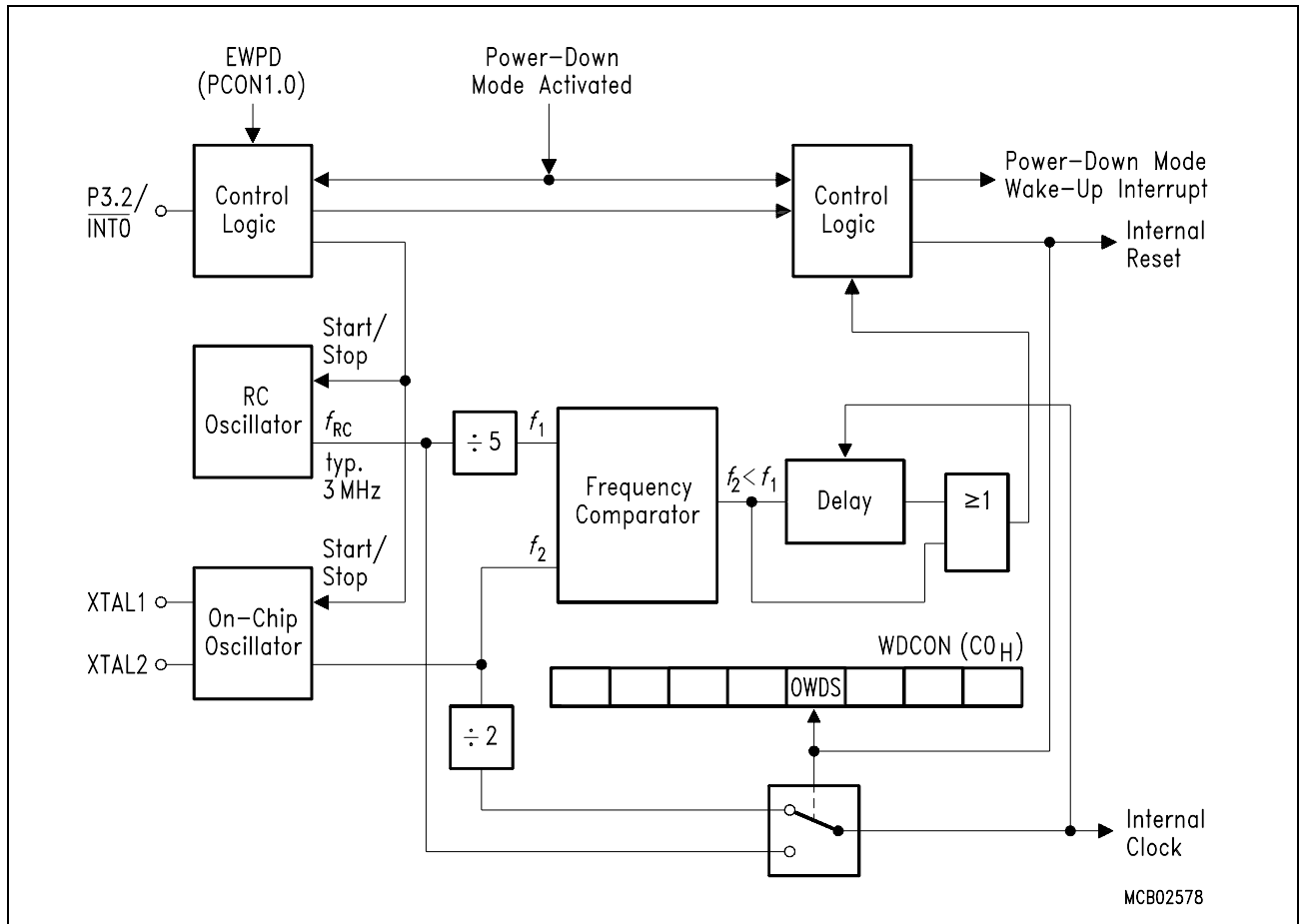
Figure 19 Block Diagram of the Oscillator Watchdog
