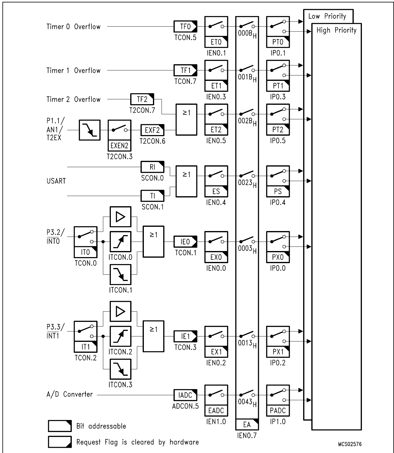
Figure 16 Interrupt Request Sources (Part 1)
