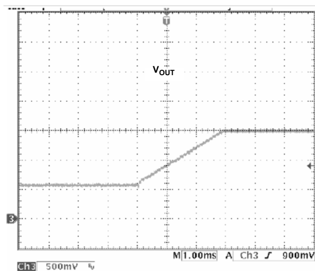
FIGURE 17. PRE-BIASED START-UP
