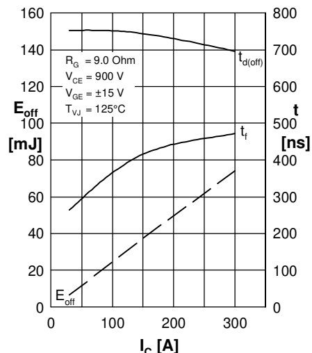
Fig. 5 Typ. turn-off energy &amp; switch. times vs. collector current
