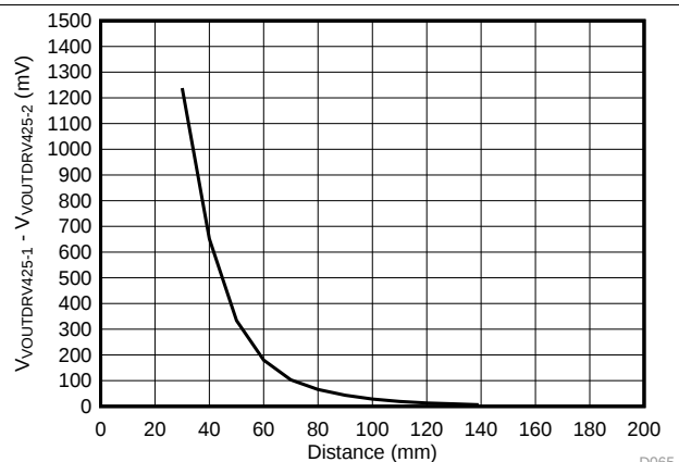
Figure 70. Difference Between Two DRV425 Outputs vs Distance to the Magnet
