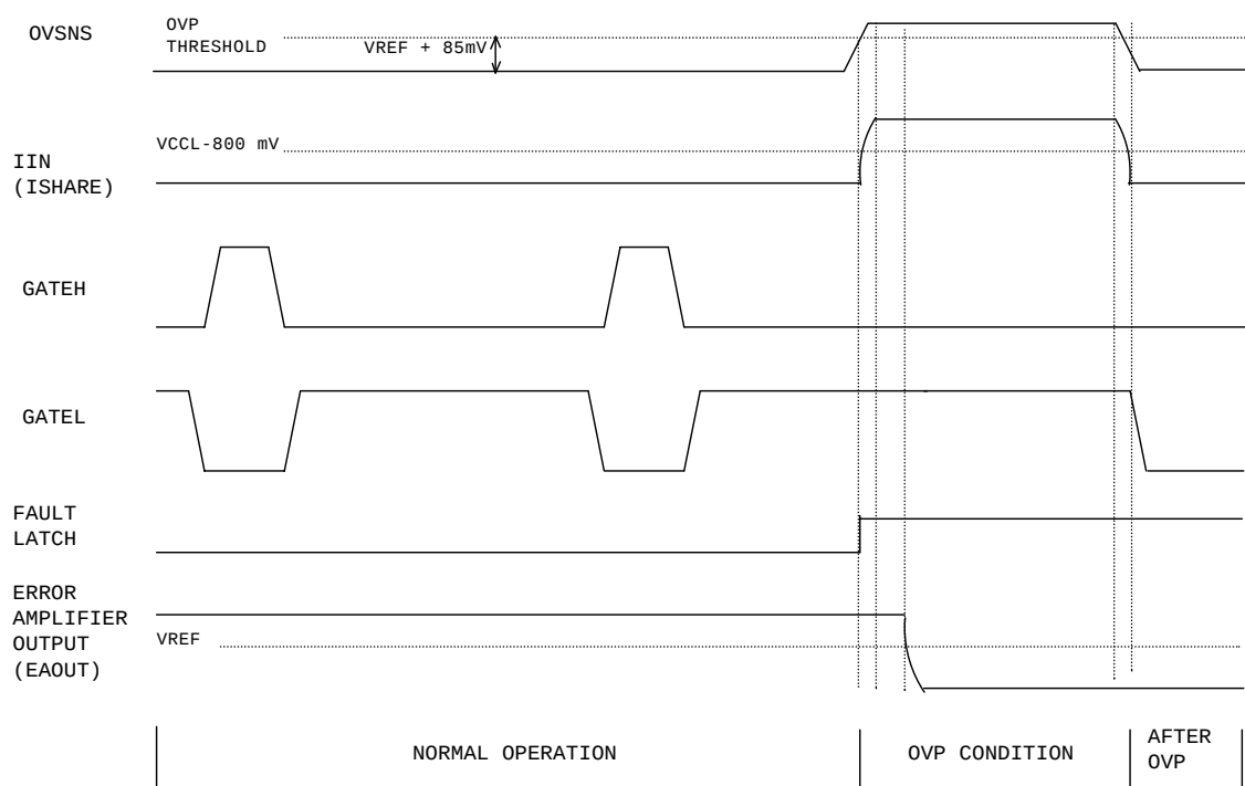
Figure 11 Over-voltage protection during normal operation
