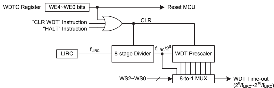
Watchdog Timer
