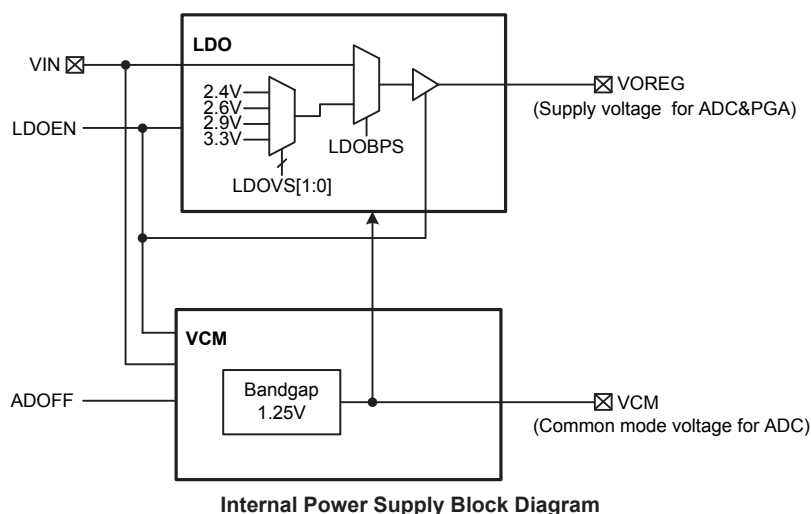
Internal Power Supply Block Diagram
