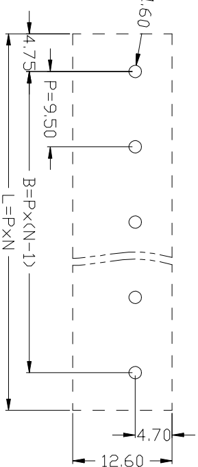
PCB LAYOUT
