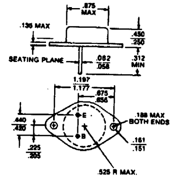
MODIFIED TO-3 (60 mil pins)
