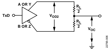
Figure 30. Driver Voltage Measurement, |V_{OD2}|
