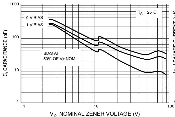
Figure 7. Typical Capacitance
