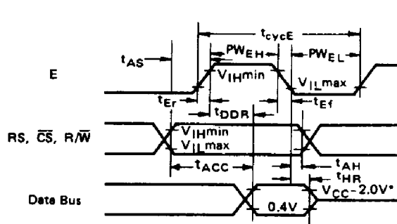
Figure 1 Bus Read Timing (Read Information from PTM)
