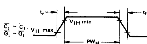
Figure 4 Input Pulse Width "High"
