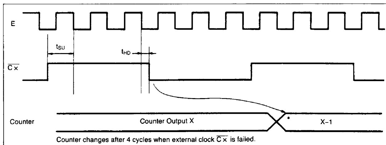
Figure A. External Clock Synchronous Timing
