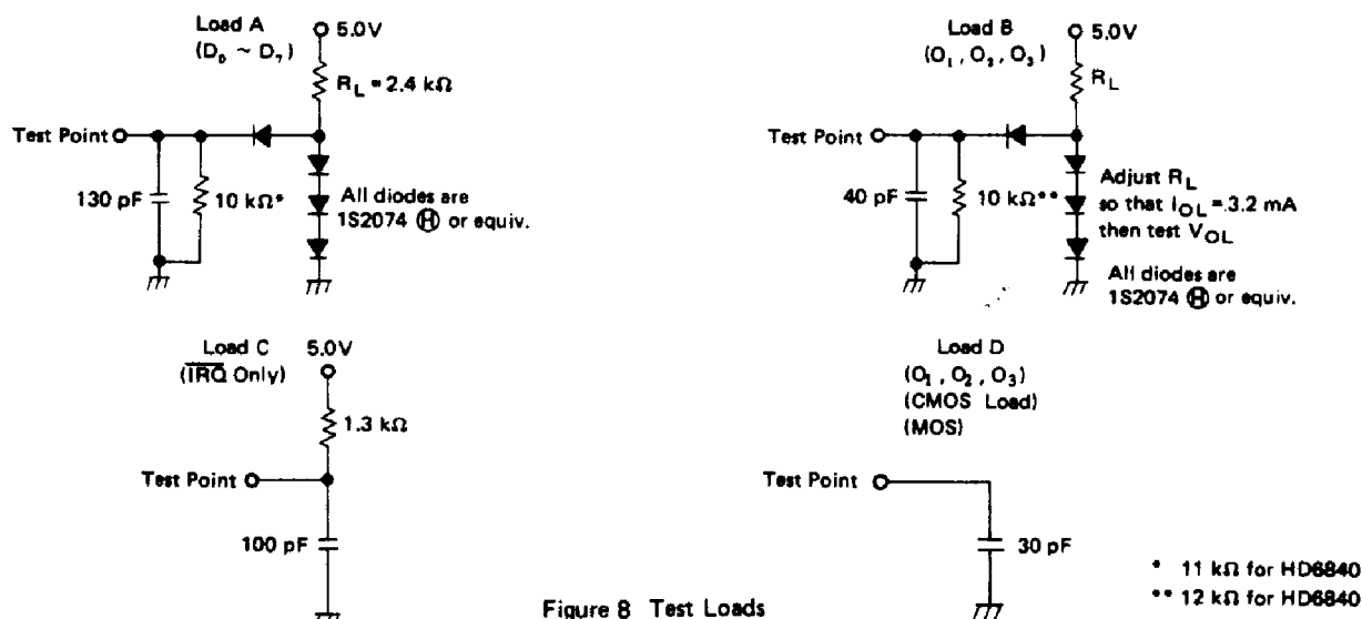
Figure 8 Test Loads
