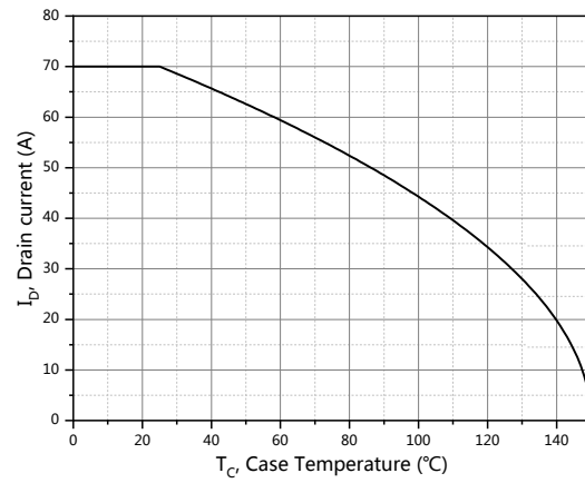
Figure 10, Drain current
