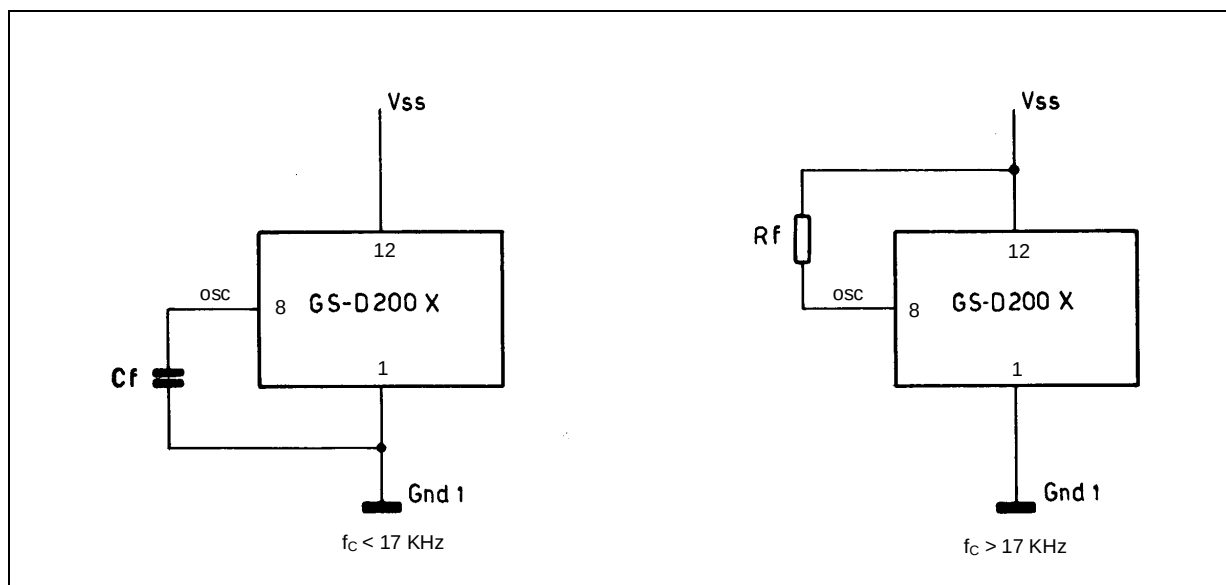
Figure 15: Chopper Frequency Programming
