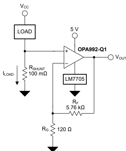
Figure 7-1. OPAx992-Q1 in a Low-Side, Current-Sensing Application
