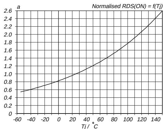
Fig.9. Normalised drain-source on-state resistance. a = R_{DS(ON)} / R_{DS(ON)25^\circ\text{C}} = f(T_j) ; I_D = 1.5 \text{ A} ; V_{GS} = 10 \text{ V}
