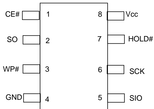
8-Pin SOIC/VVSOP
