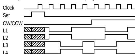
Figure 6. Timing Diagram
