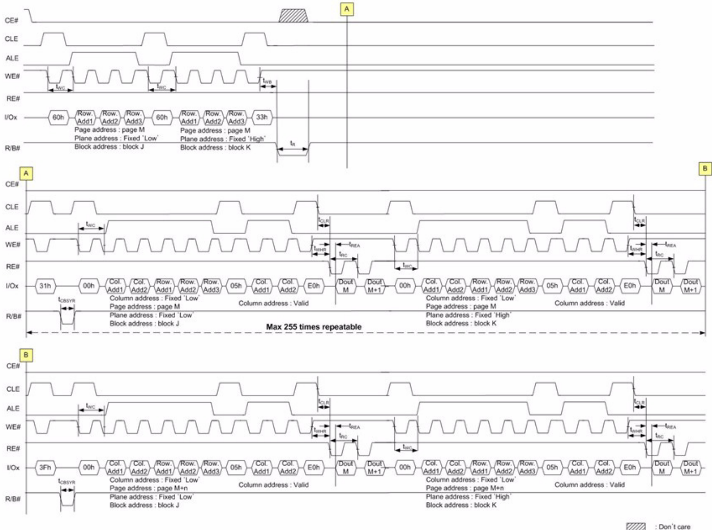
■ Figure 20. Multi plane cache read operation Timings
