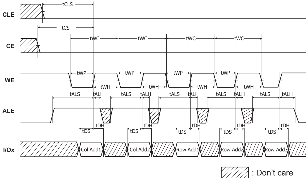
■ Figure 8. Address latch timings
