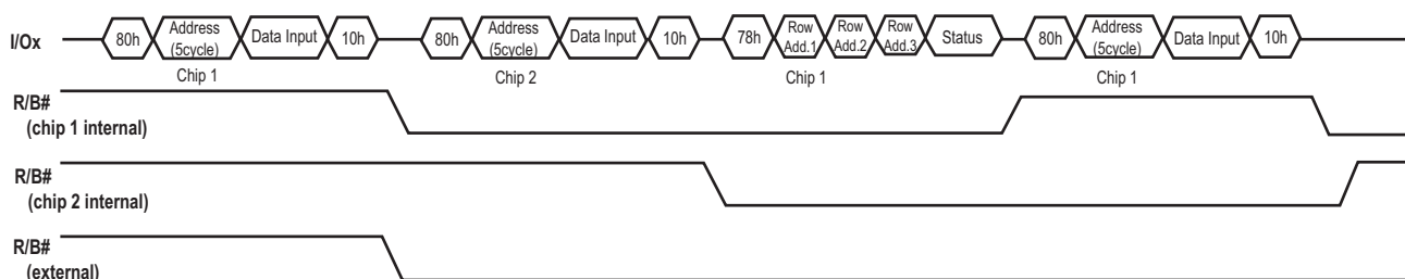
■ Figure 53. Interleaved page program
