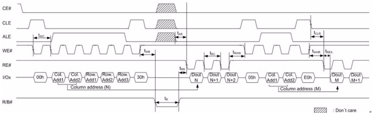
■ Figure 17. Random data output timings
