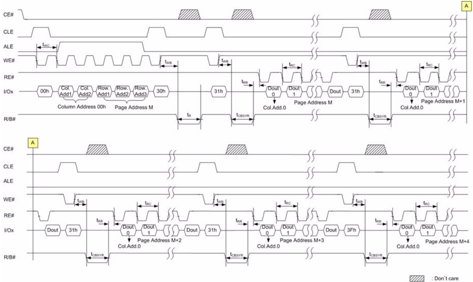
■ Figure 19. Cache read operation timings
