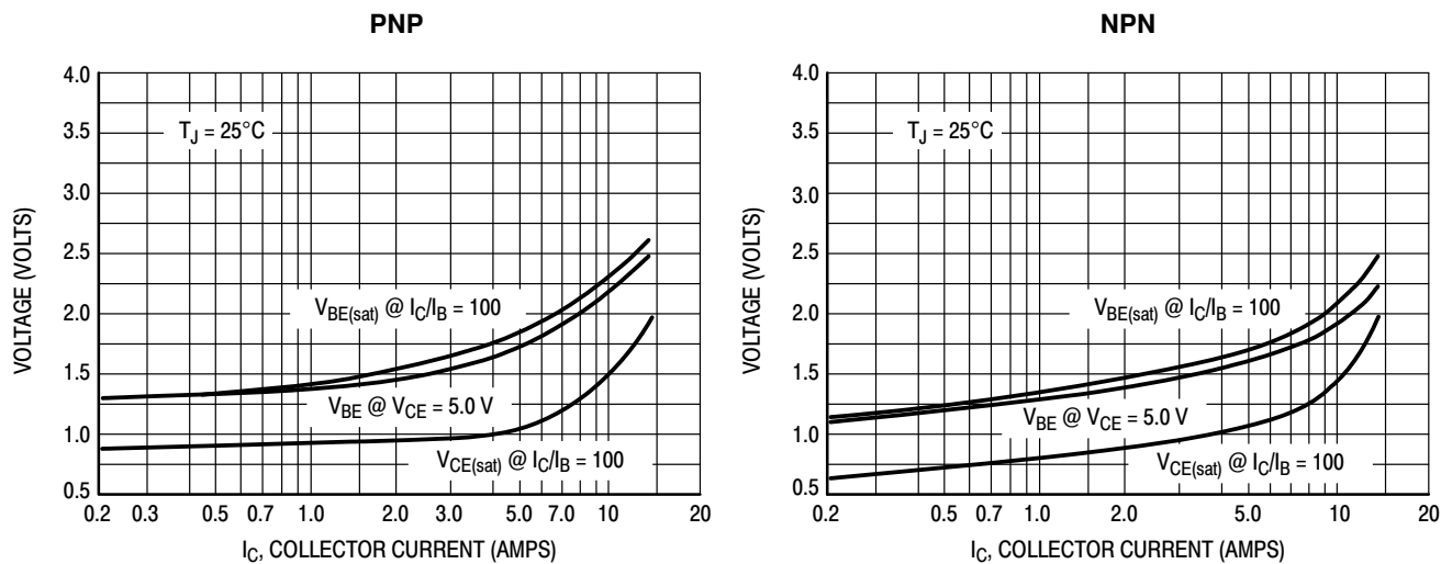
Figure 8. "On" Voltages
