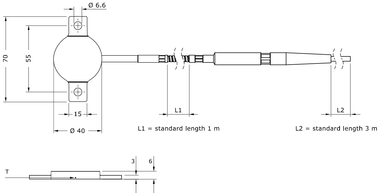
Figure 3.1.1 IHF01 industrial heat flux sensor dimensions in \times 10^{-3} \text{ m} . T marks the location of the temperature measurement
