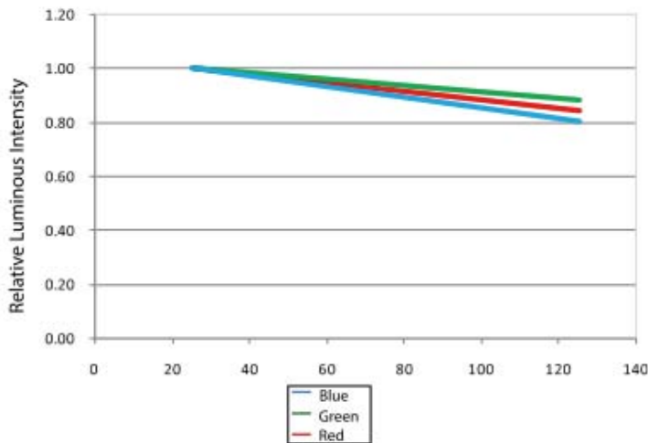
Relative Luminous Intensity vs. Junction temperature
