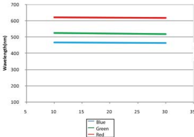
Wavelength vs. Forward Current
