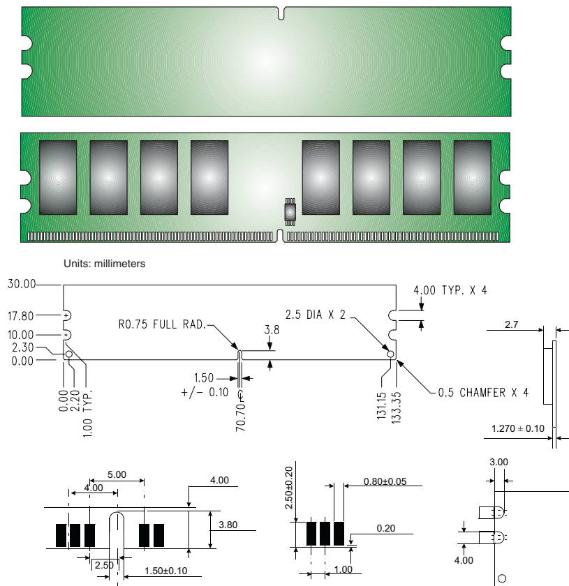
Figure 1: KVR667D2N5/512 240-Pin DIMM
