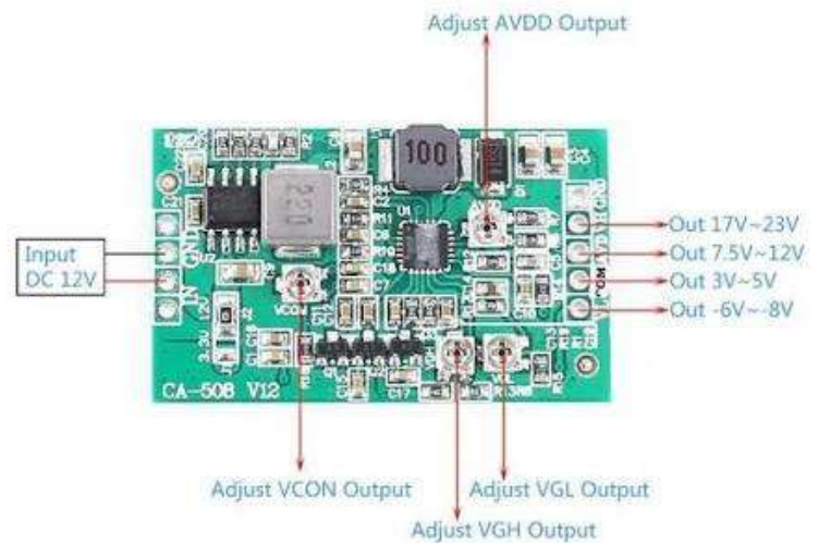
CA-508 12V Boost board module
