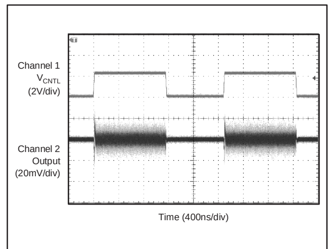
Figure 37. Response to Step Change of V_{\text{CTL}}
