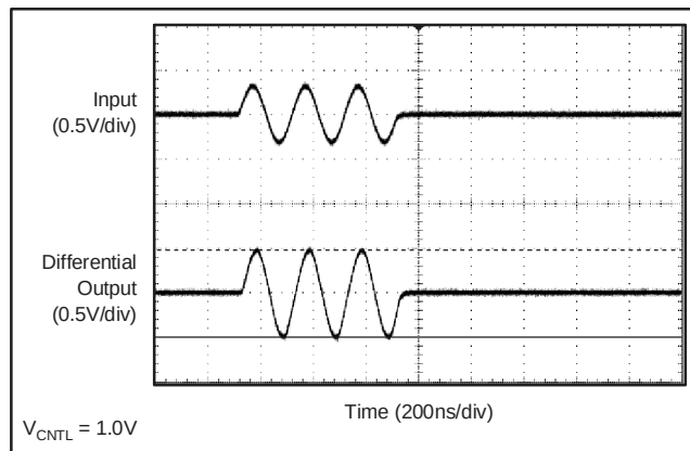
Figure 40. Before Overload (630mV PP Input)
