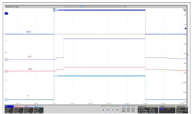
Figure 8-32. Glitch-free Power up/down- Profibus Mode
