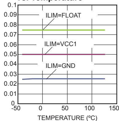
Internal Current Limit vs. Temperature
