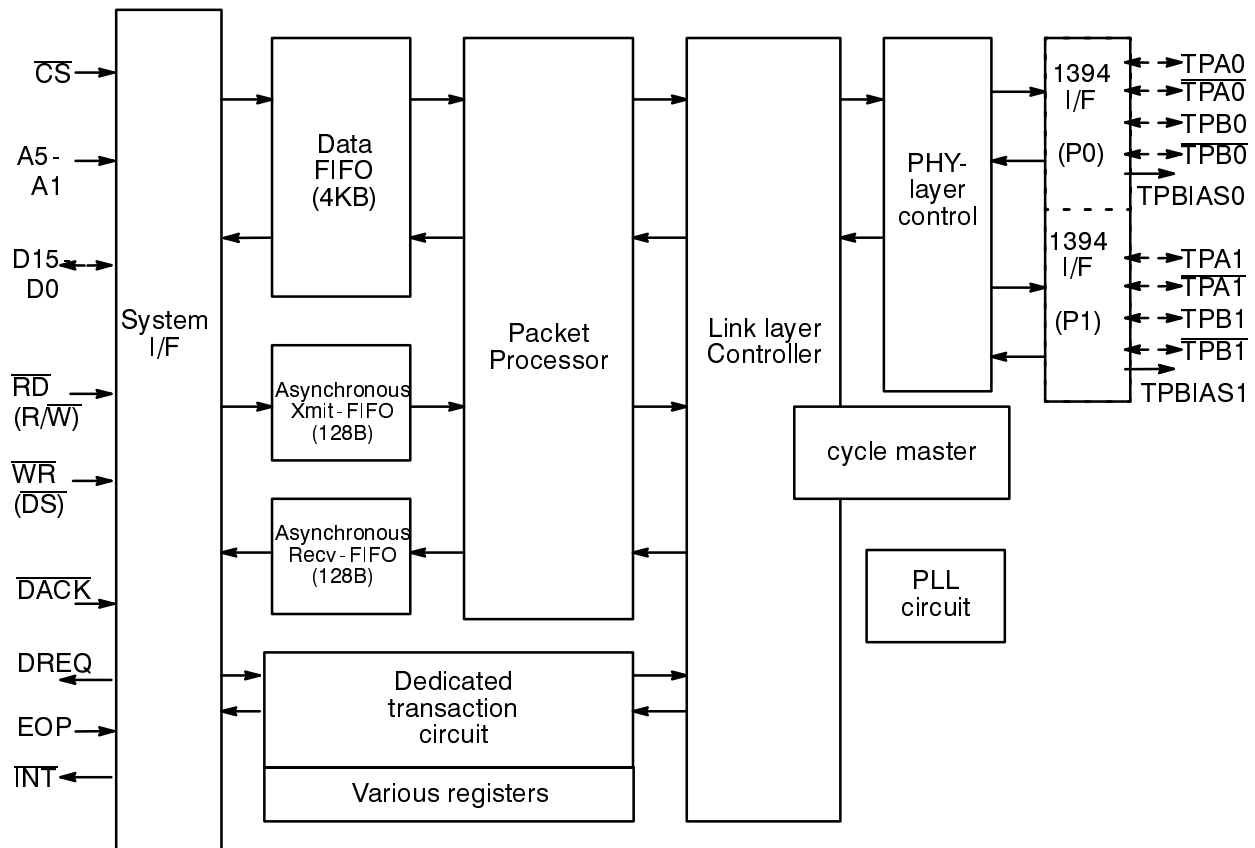
Fig. 1.1 Block Diagram
