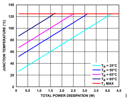
Figure 55. SOIC, T_A = 25^\circ\text{C}
