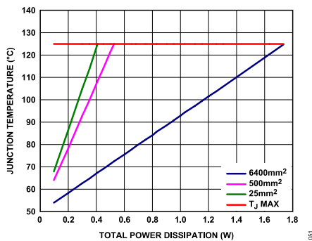
Figure 54. LFCSP, T_A = 85^\circ\text{C}
