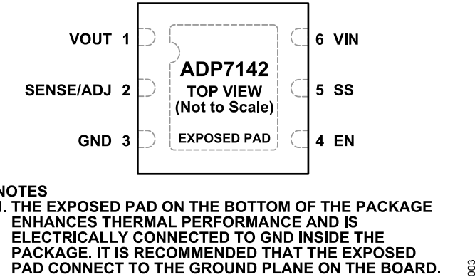
Figure 3. 6-Lead LFCSP Pin Configuration
