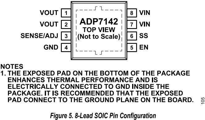
Figure 5. 8-Lead SOIC Pin Configuration
