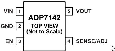
Figure 4. 5-Lead TSOT Pin Configuration
