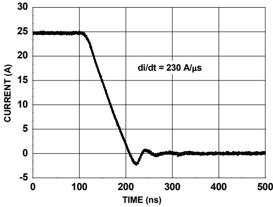
Figure 27. FDPC5030SG SyncFET™ Body Diode Reverse Recovery Characteristic
