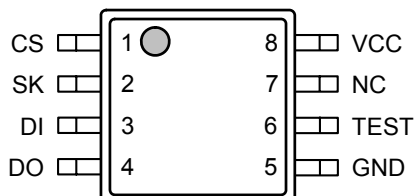
TMSOP-8 Top view
