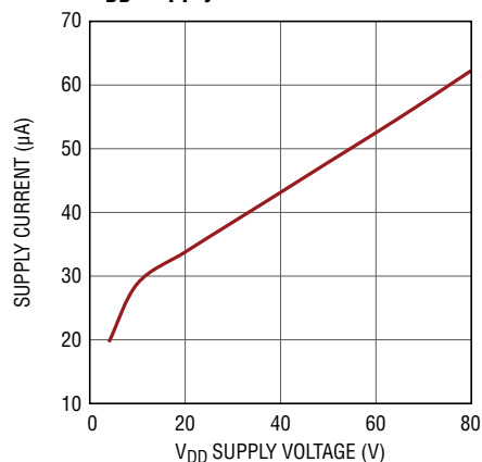
V_{DD} Supply Current in Shutdown
