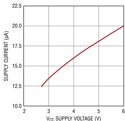
INTV_{CC} Supply Current in Shutdown
