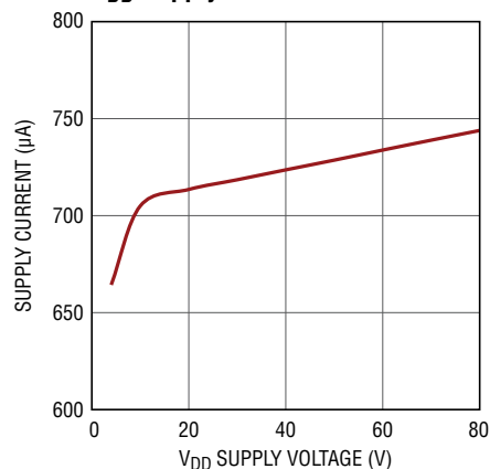
V_{DD} Supply Current
