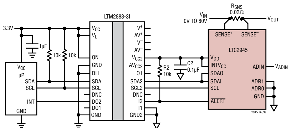
Isolated Wide Range I 2 C Power Monitor
