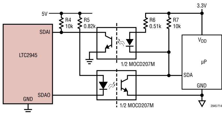
Figure 14. Opto-Isolation of a 10kHz I²C Interface Between LTC2945 and Microcontroller (SCL Omitted for Clarity)
