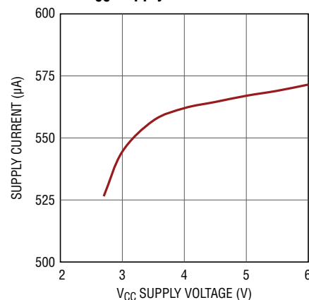
INTV_{CC} Supply Current
