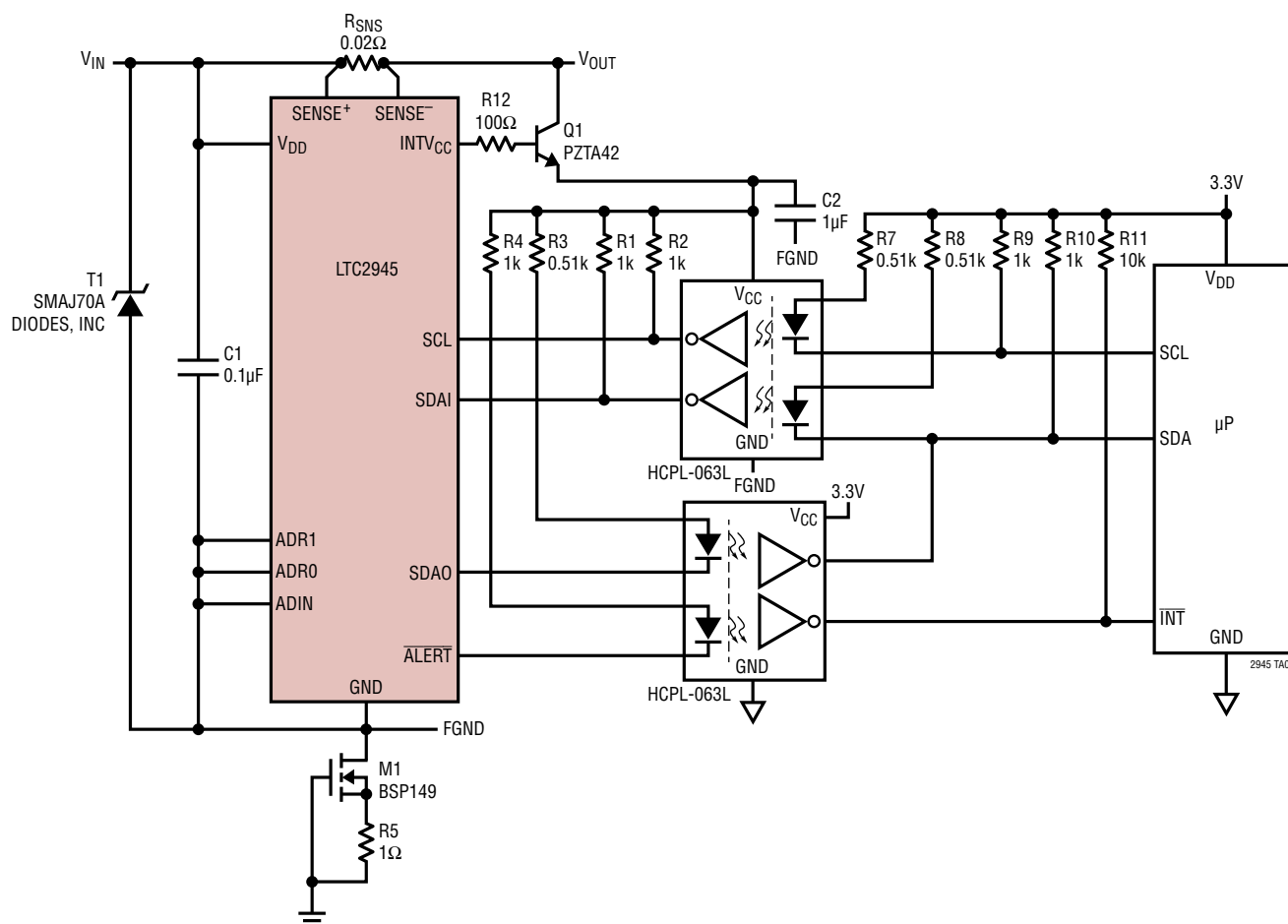
Ruggedized 4V to 70V High Side Power Monitor with Surge Protection Up to 200V
