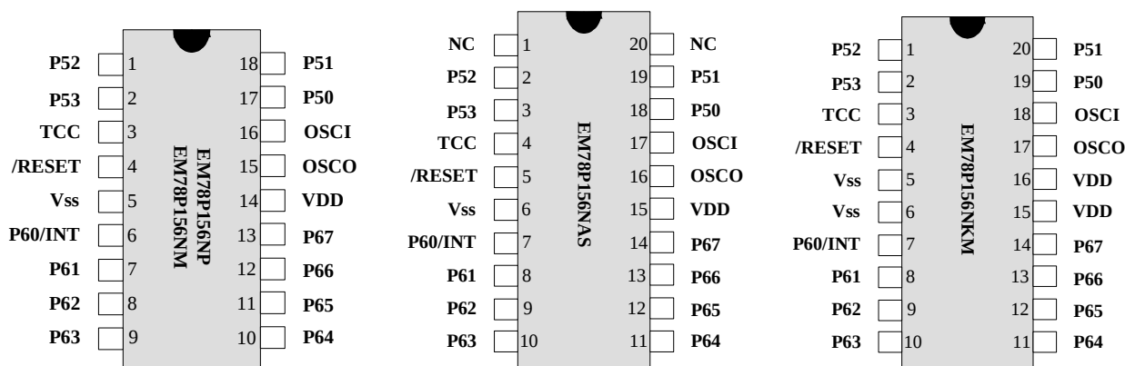
Fig. 1 Pin Assignment
