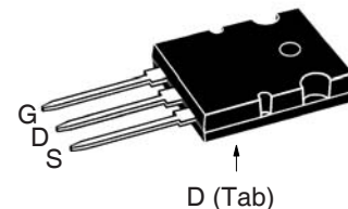
TO-264 (IXTK)
