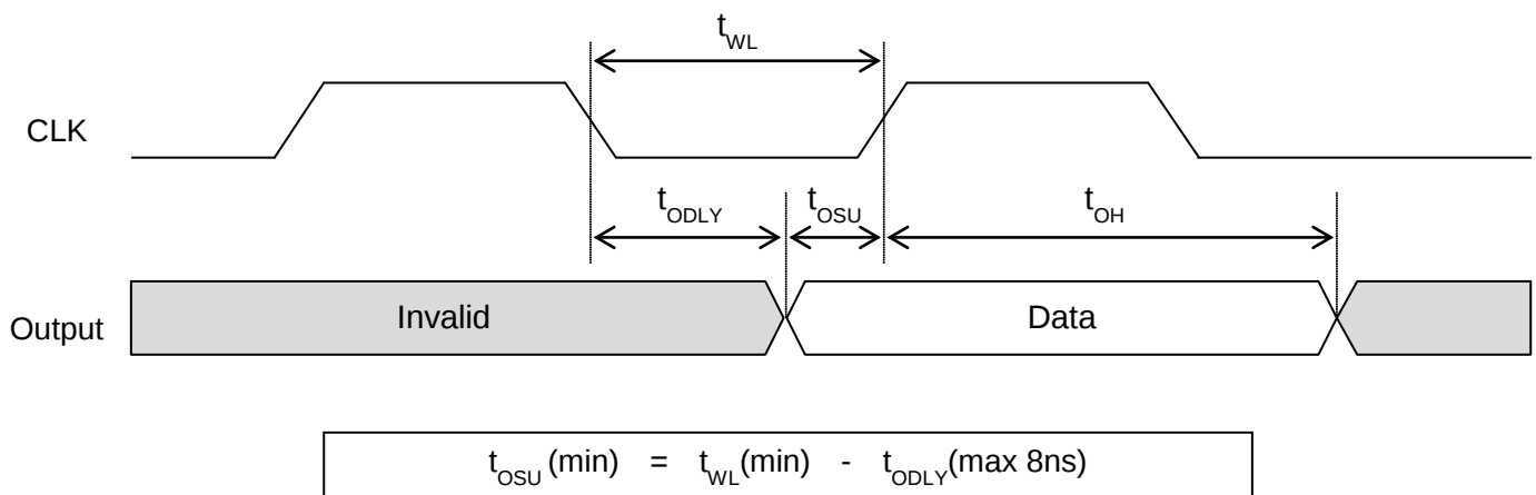
Figure 2 Output timing
