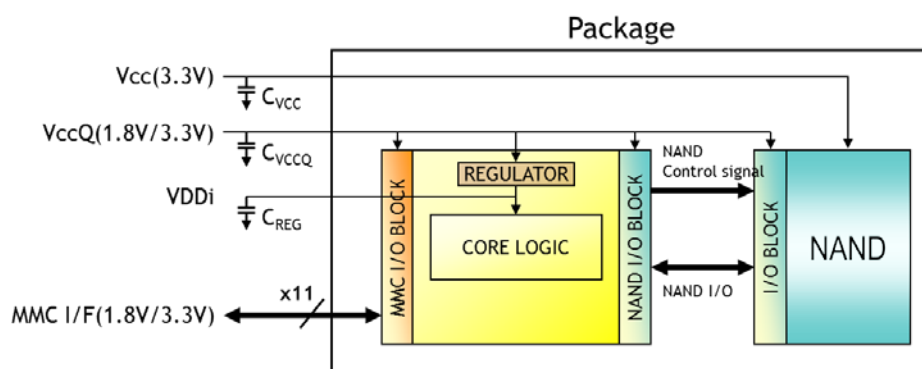
Figure 1 THGBMBG7D2KBAIL Block Diagram
