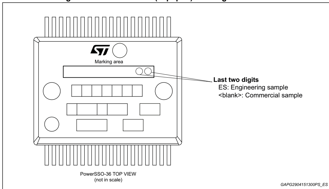
Figure 18. PowerSSO-36 (exp. pad) marking information
