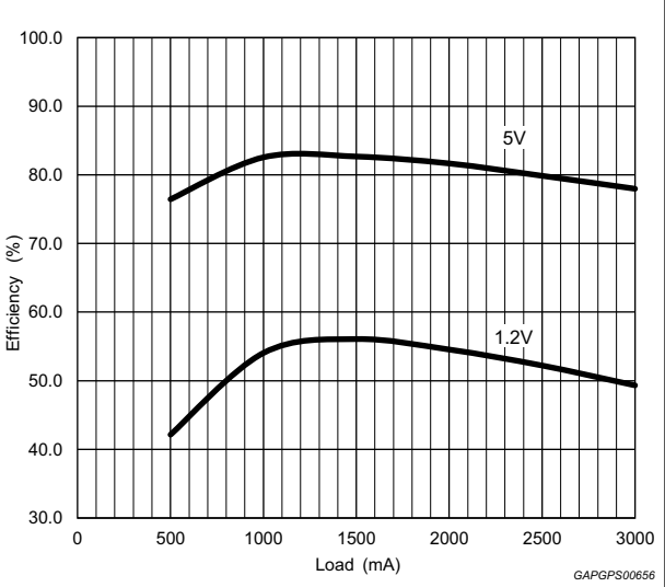
Figure 6. Efficiency vs. output current (VIN = 14 V, fsw = 2 MHz)
