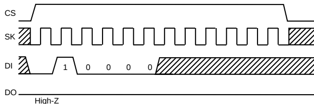
Fig.6 Write disable cycle timing (WDS)
