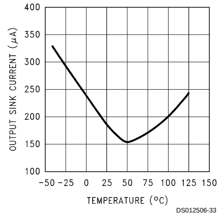
Output Reverse Leakage vs Temperature
