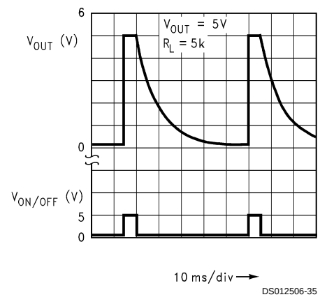
Turn-Off Waveform
