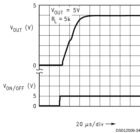
Turn-On Waveform
