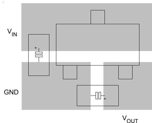
SOT-23 Board Layout
