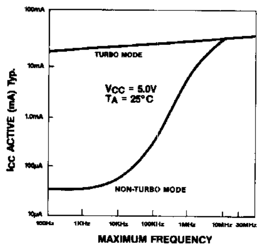
Figure 2. I_{CC} vs Frequency
