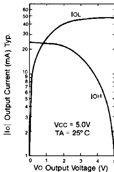
Figure 3. Output Drive Currents
