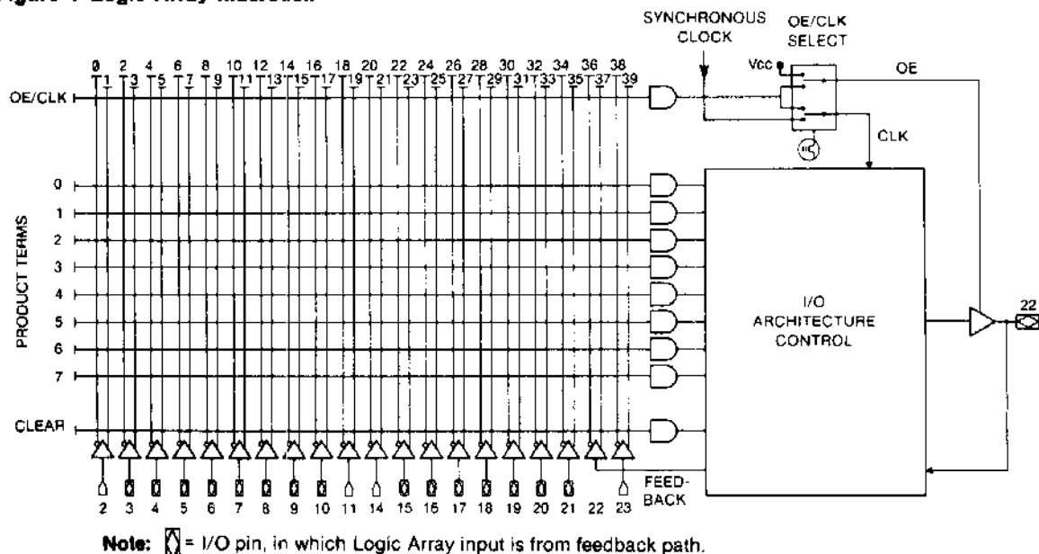
Figure 1 Logic Array Macrocell
