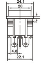
KCD1-201-6 ON-OFF KCD1-201N-6 ON-OFF KCD1-202-6 ON-OFF KCD1-202N-6 ON-ON KCD1-203-6 ON-OFF-ON
