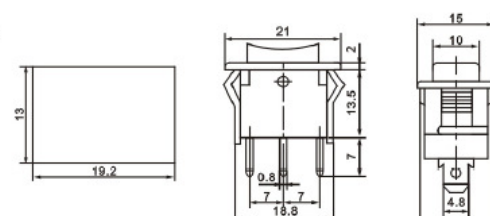
KCD1-103-2 ON-OFF-ON KCD1-123-2 (ON)-OFF-(ON) (双复位)
