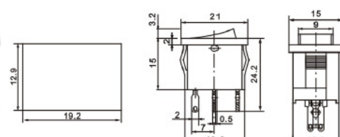
KCD1-103-2 ON-OFF-ON KCD1-123-2 (ON)-OFF-(ON) (双复位)
