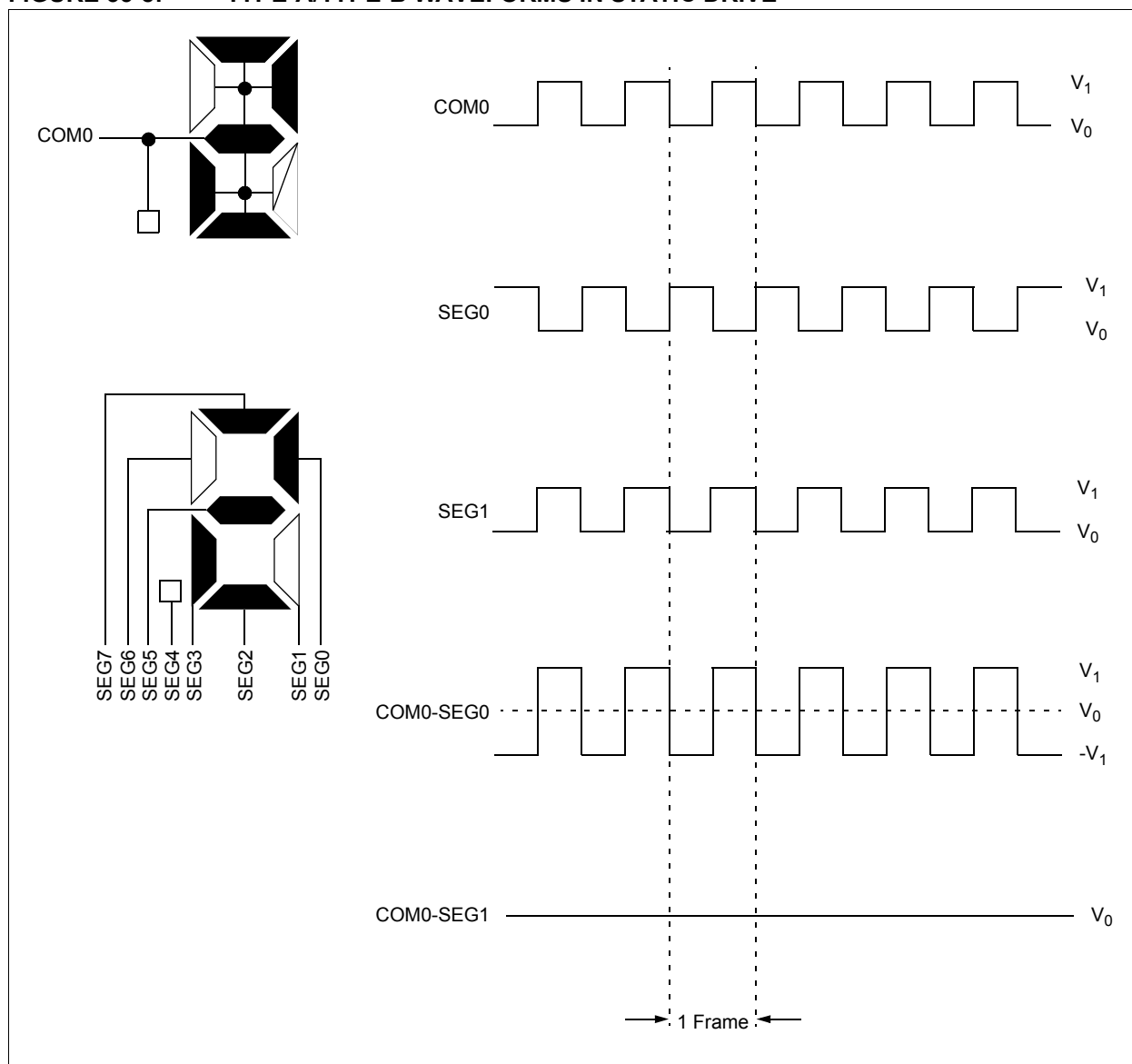
FIGURE 35-8: TYPE-A/TYPER-B WAVEFORMS IN STATIC DRIVE
