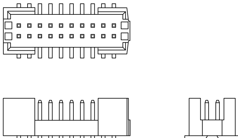
Figure 2.2 Header Pin Dimensions
