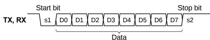
Figure 5.4 UART Bit Format
