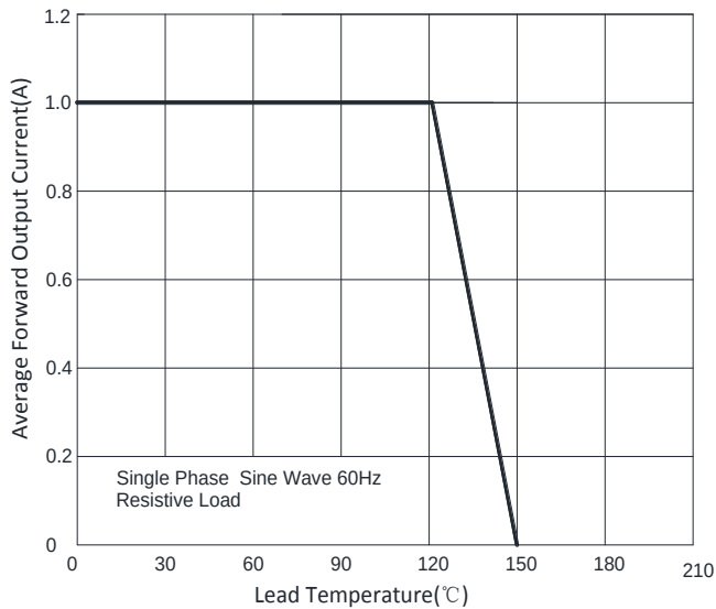
FIG1: Io-TL Curve
