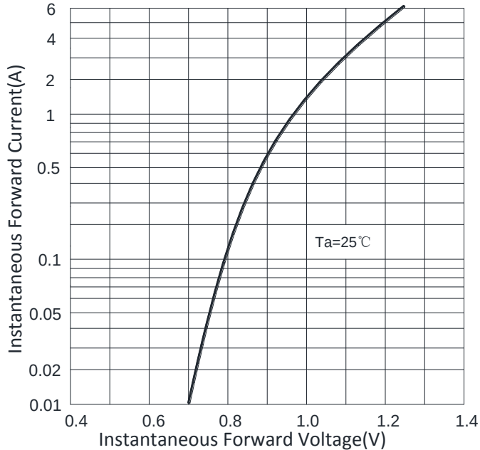
FIG3: Forward Voltage
